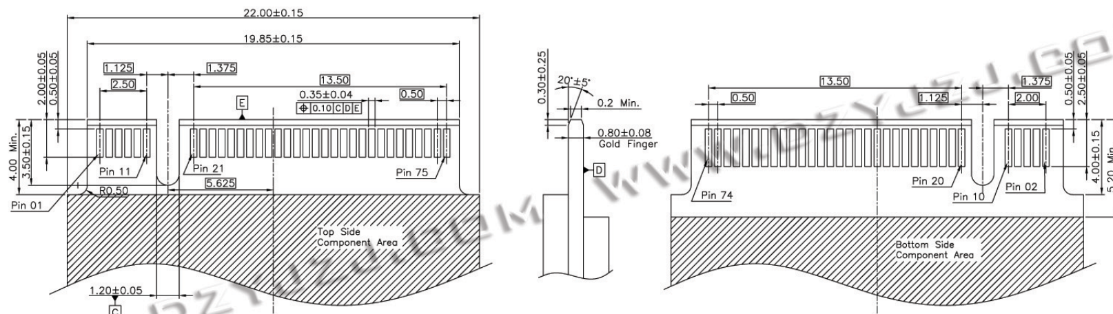
Recommended Module Finger Layout
